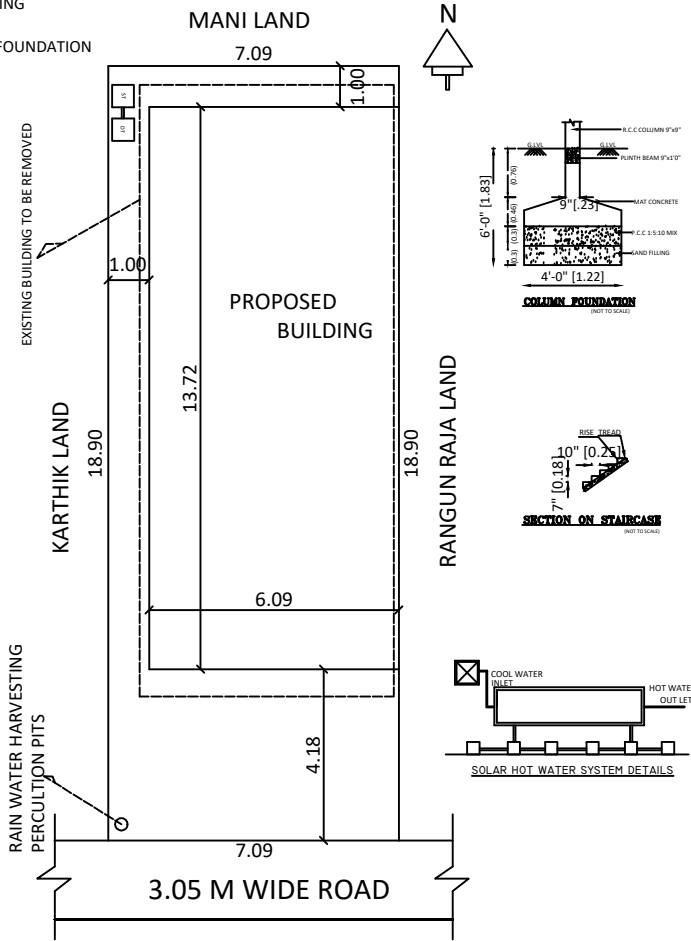
SITE PLAN
