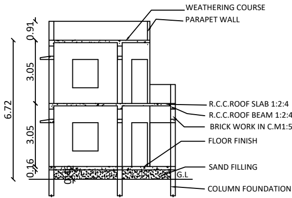
SECTION- SS
