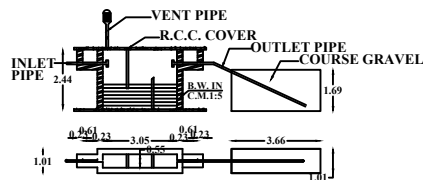
SEPTIC TANK & OF DISPERSION TRENCH DETAILS
