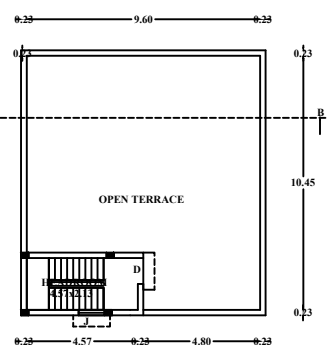
FLOOR-TERACE
