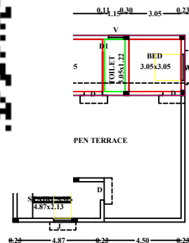
FLOOR01
