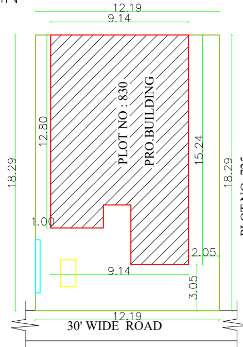
SITE PLAN
