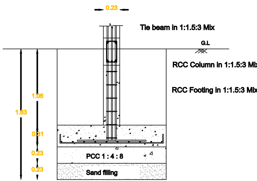
FOUNDATION DETAILS
