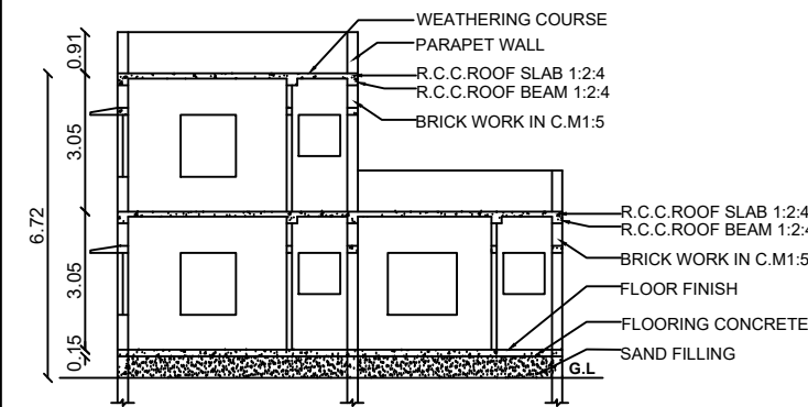
SECTION ON SS
