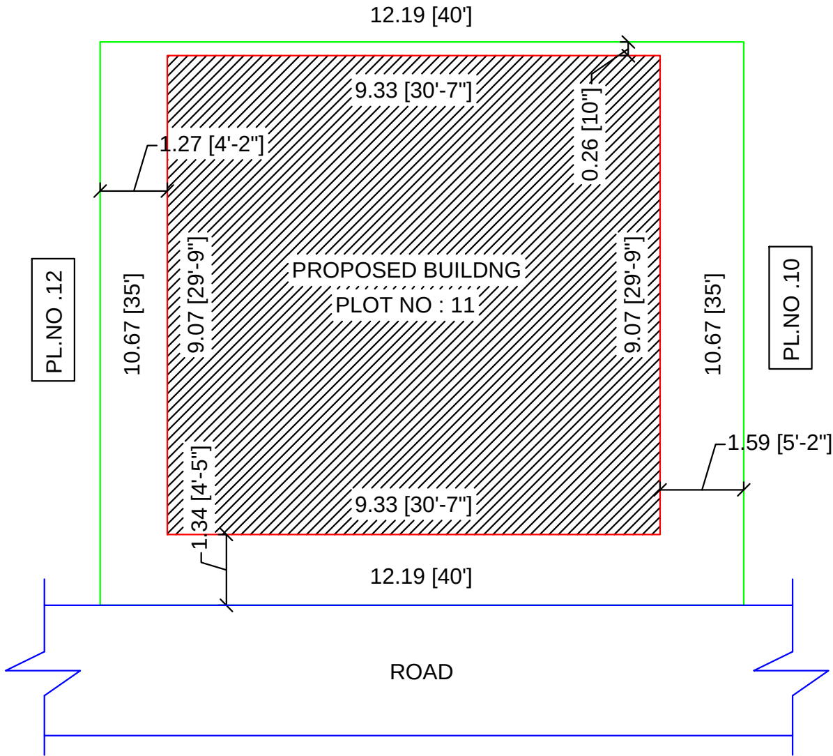
SITE PLAN
