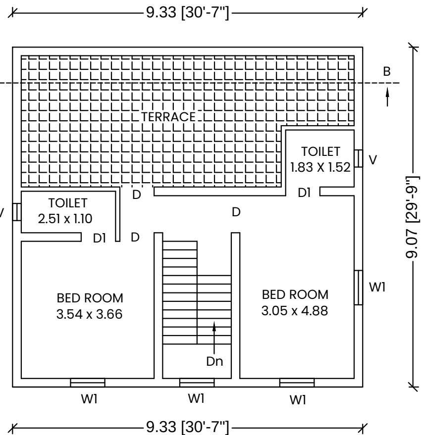
FIRST FLOOR PALN
