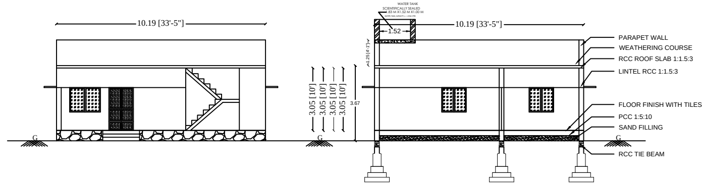
FRONT ELEVATION
