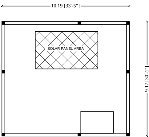
OPEN TERRACE PLAN
