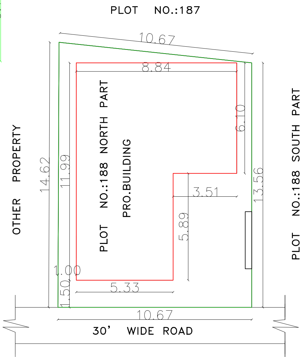
SITE PLAN
