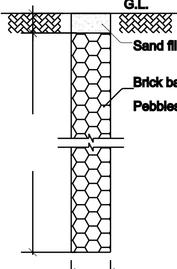
Percolation Pit
