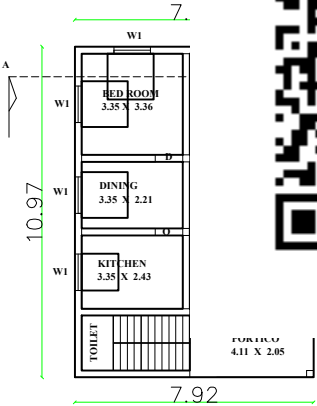
FLOOR- GROUND
