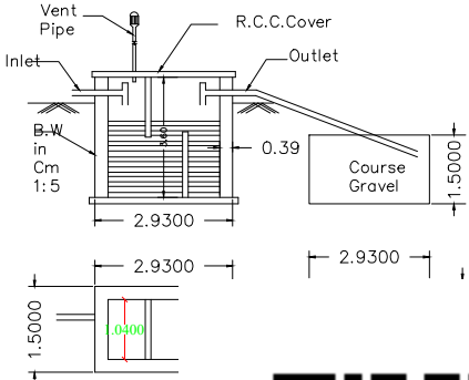
SEPTIC TANK
