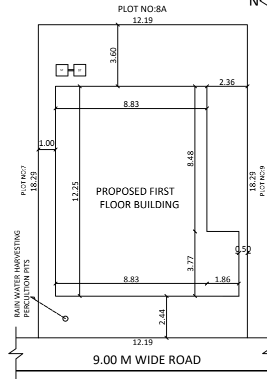
SITE PLAN
