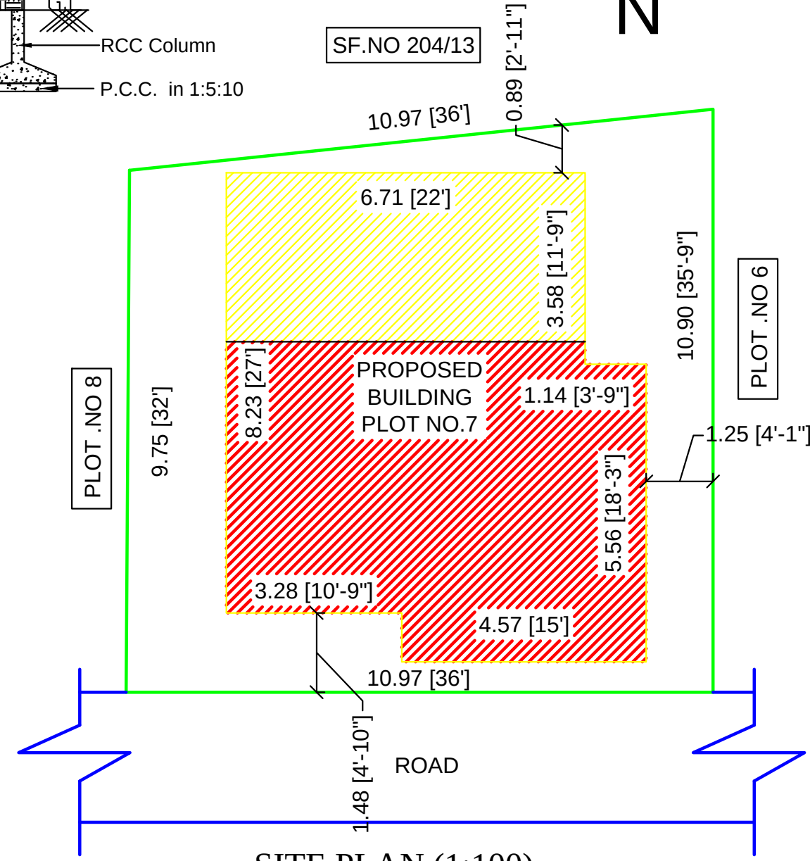
SITE PLAN (1:100)
