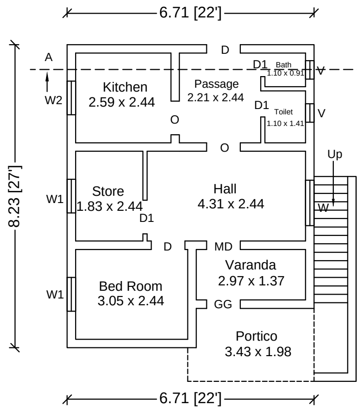
EX.GROUND FLOOR PLAN
