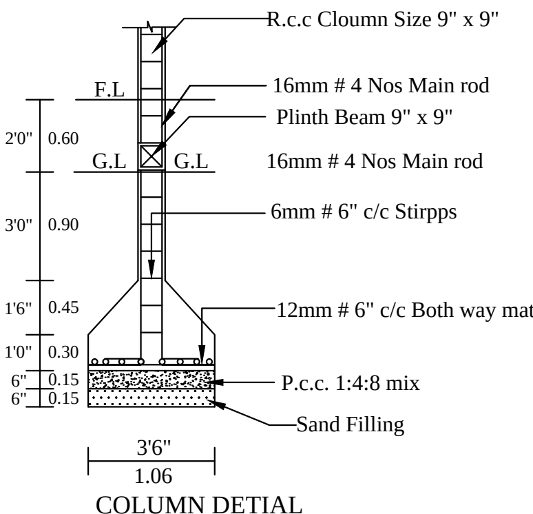
COLUMN DETIAL
