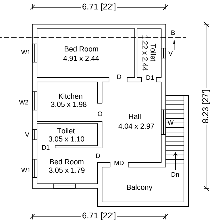
EX & PROPOSED FIRST FLOOR PLAN
