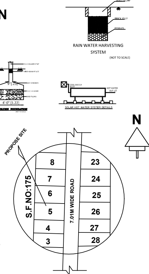
LOCATION PLAN
