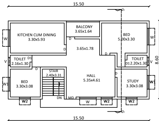
FIRST FLOOR PLAN (PRO)
