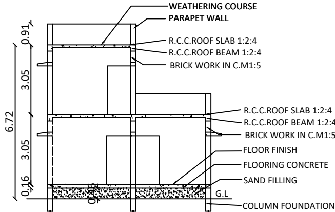
SECTION ON GG
