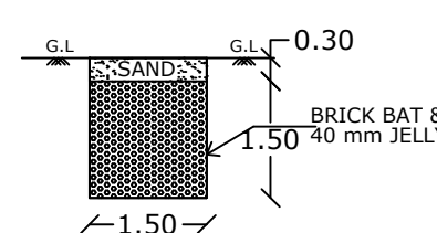
RAIN WATER HARVESTING SYSTEM ( Scale 1:100 )
