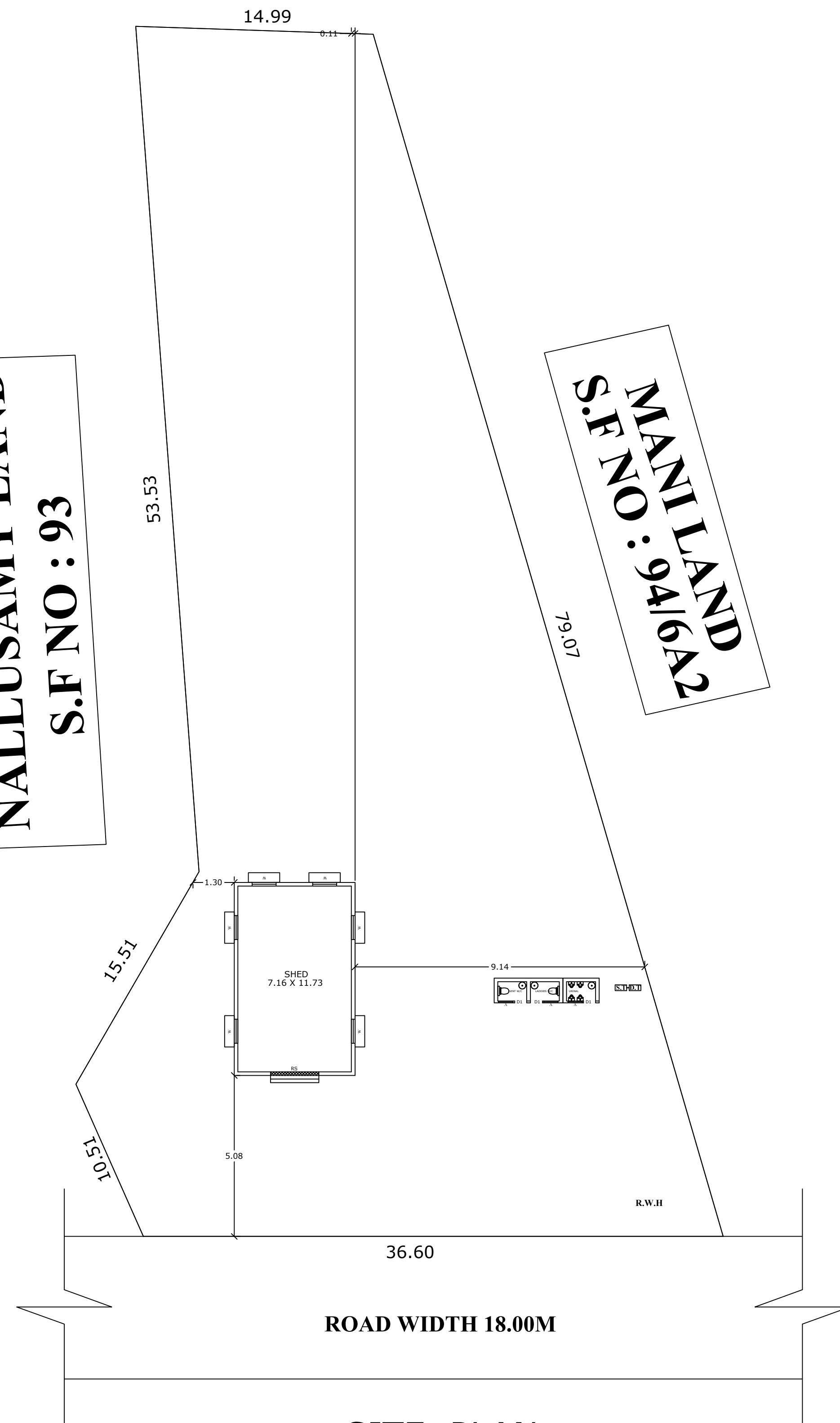
SITE PLAN ( Scale 1m:4m )
