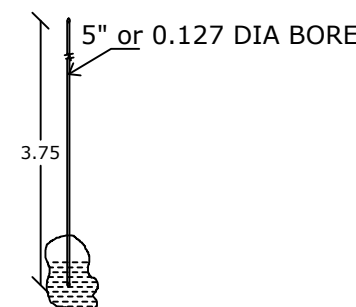
BORE WELL ( Scale : 1m:4m )
