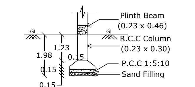
FOUNDATION DETAILS ( Scale 1:100 )
