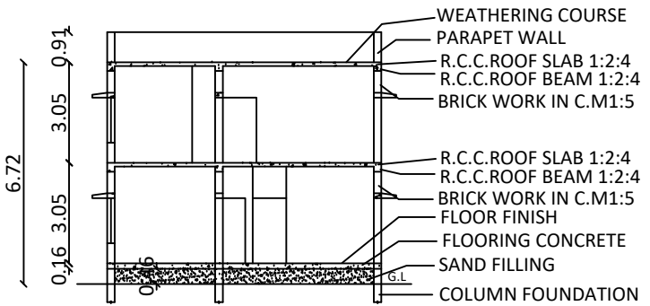
SECTION- SS
