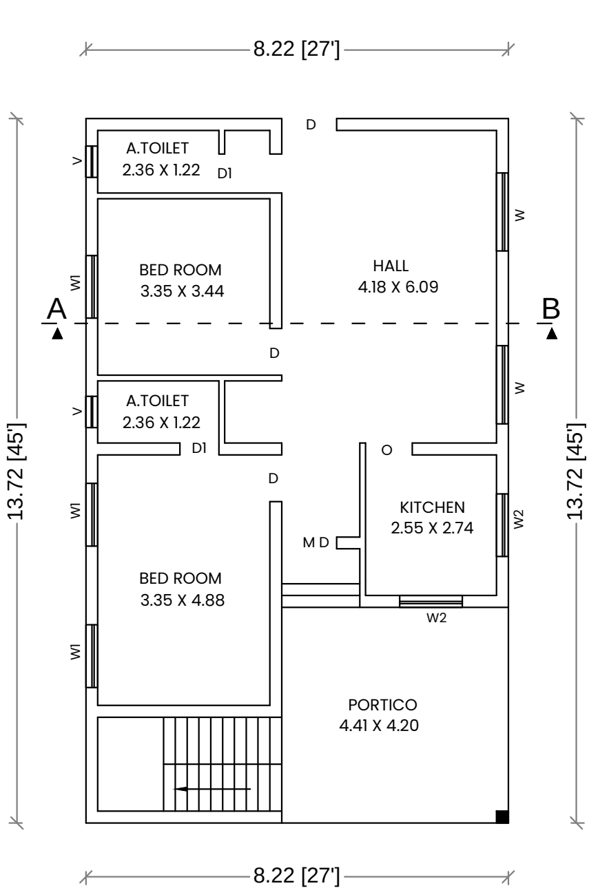
PLAN
