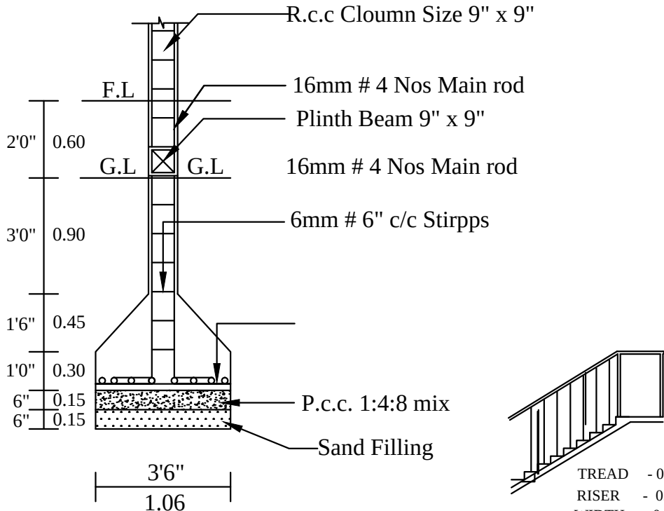
COLUMN DETIALS
