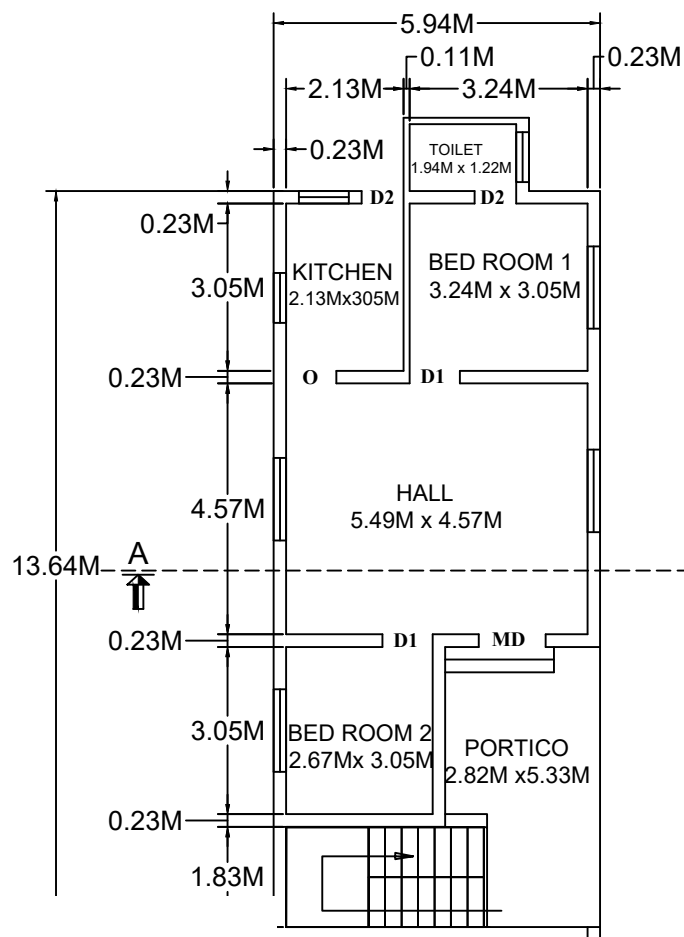
SED GROUND FLOOR PLAN
