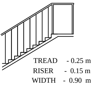
STAIRCASE DETAILS
