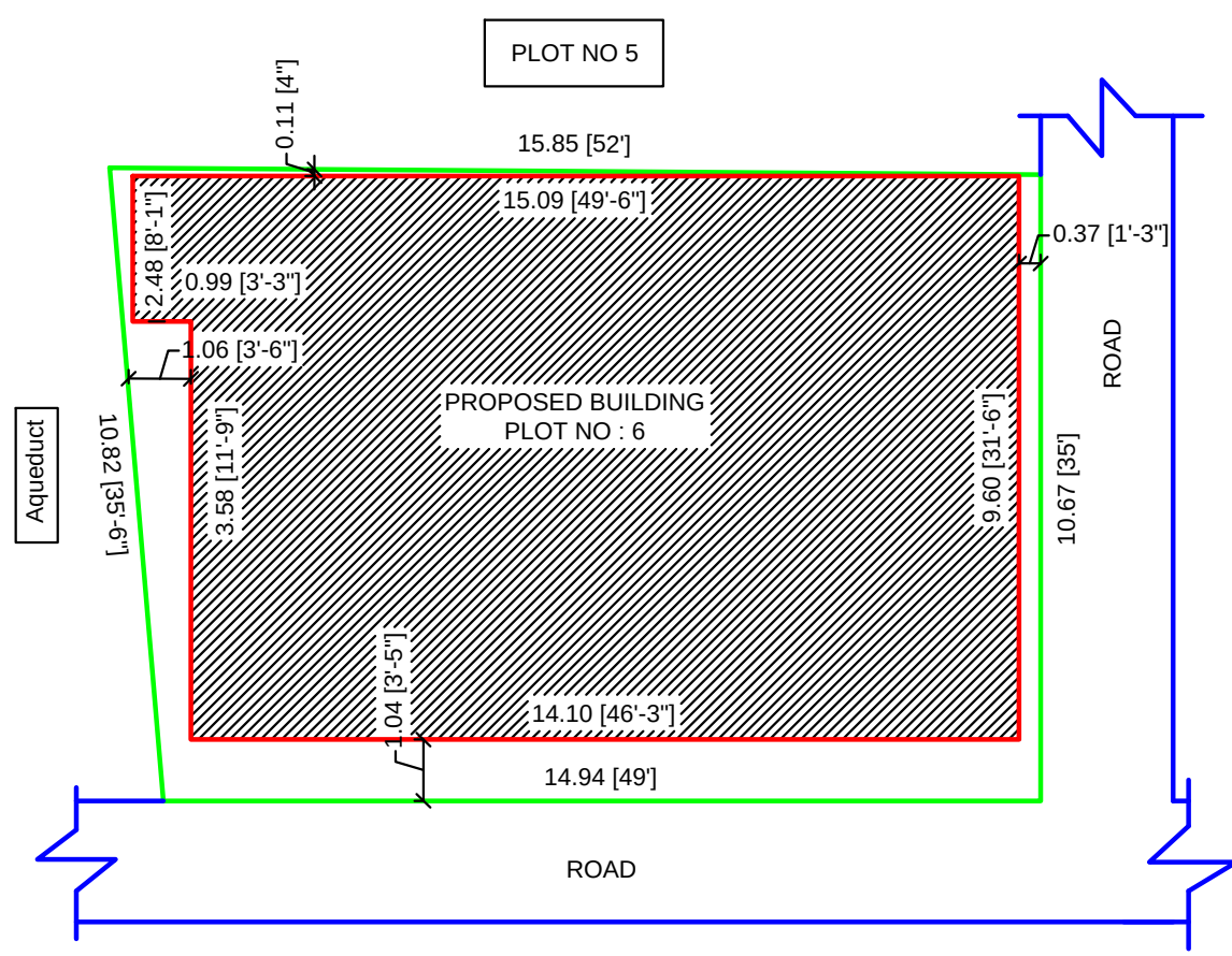
SITE PLAN (1:100)
