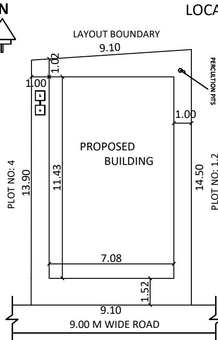
SITE PLAN
