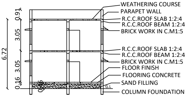
SECTION- SS
