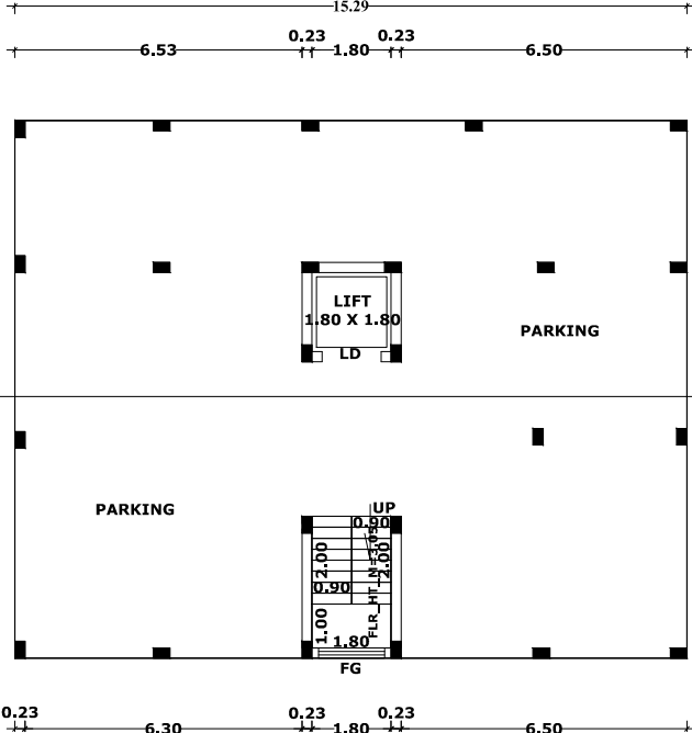
STILT FLOOR PLAN
