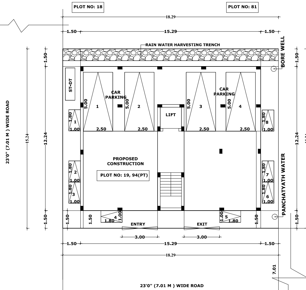
SITE PLAN
