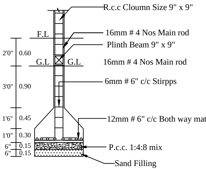
COLUMN DETAILS
