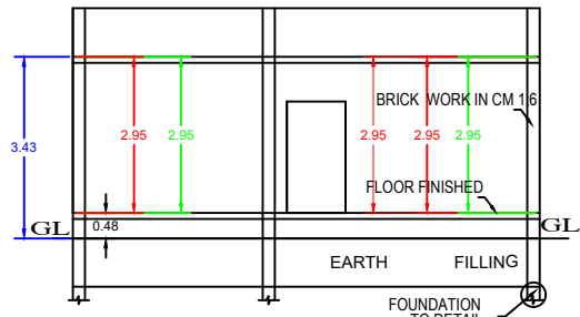
SECTION "A-B"
