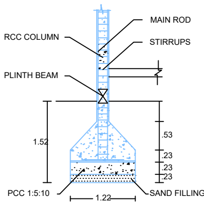
COLUMN DETAILS
