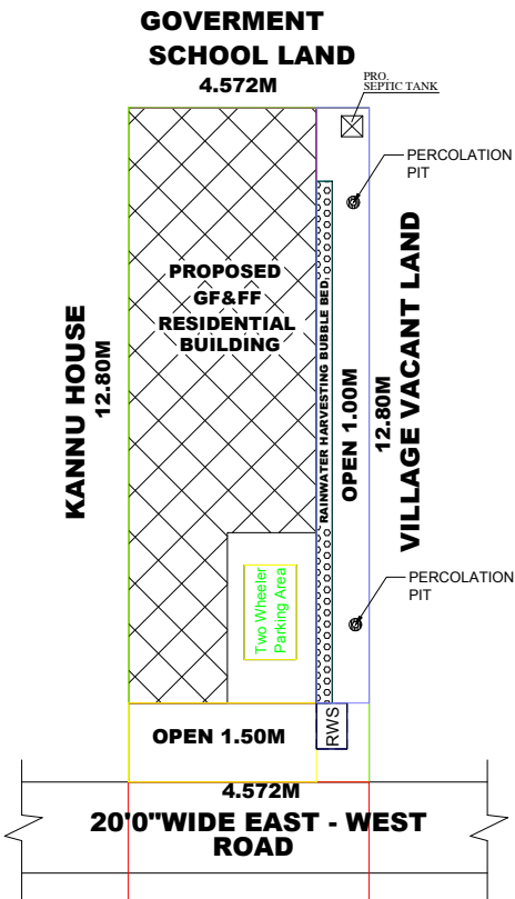
SITE PLAN (SCALE 1:1)
