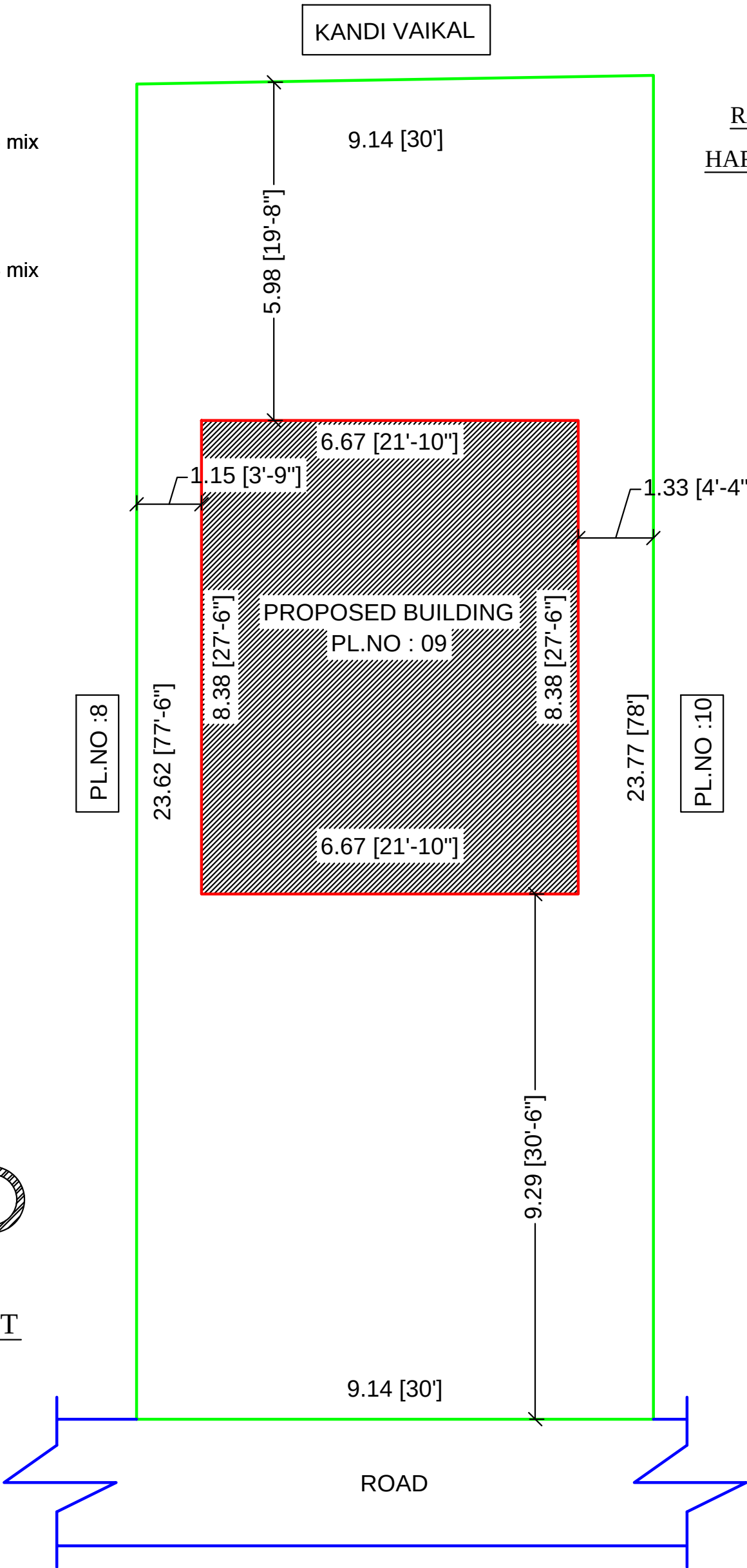
SITE PLAN
