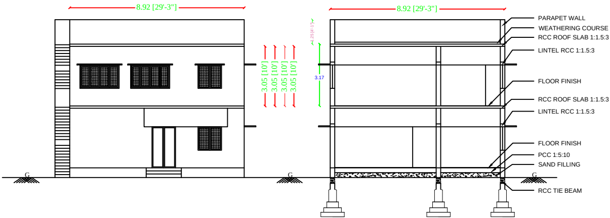
FRONT ELEVATION
