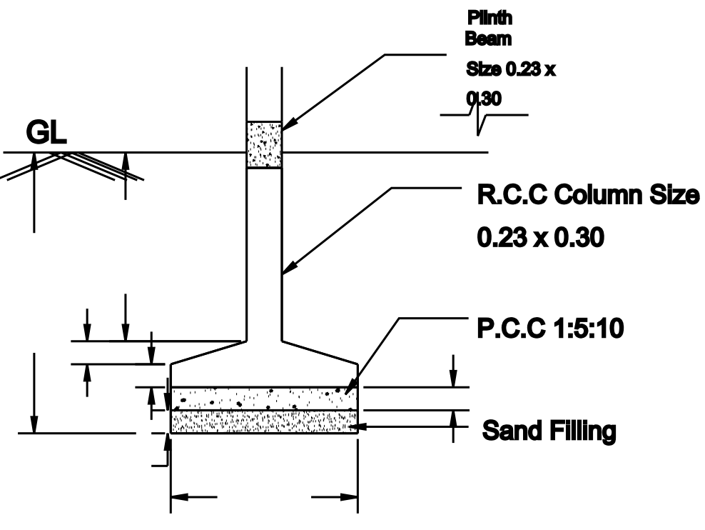
FOUNDATION DETAILS
