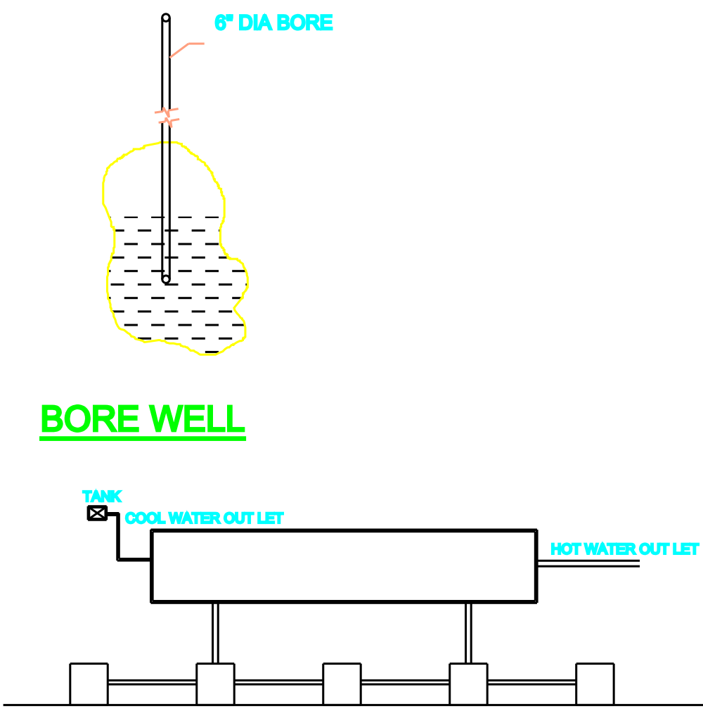
SOLAR HOT WATER SYSTEM DETAILS
