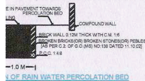
DETAIL OF RAIN WATER PERCOLATION BED
