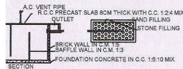
PLAN & SECTION OF SEPTIC TANK & DISPERSION TRENCH
