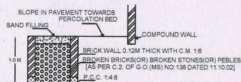
FOUNDATION DETAILS
