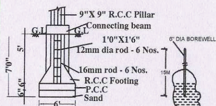
FOUNDATION DETAILS
