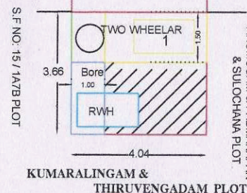
SITE PLAN
