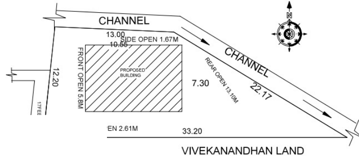
E PLAN
