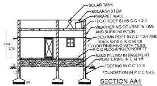
SECTION AA1
