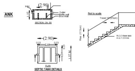
SEPTIC TANK DETAILS
