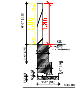
COMPOUND WALL
