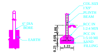
BORE WELL
