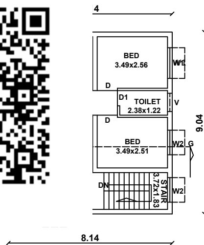
FIRST FLOOR PLAN (PRO)
