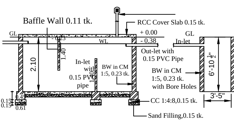
SECTION - SEPTIC TANK & SOAK PIT
