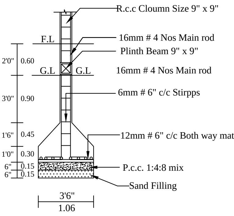
COLUMN DETIAL
