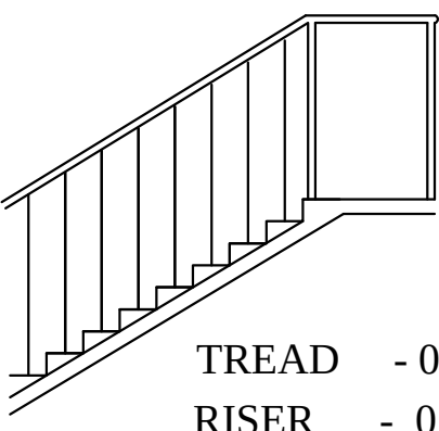
STAIRCASE DETAILS
