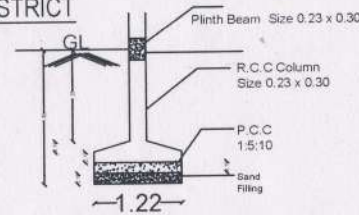
FOUNDATION DETAILS
