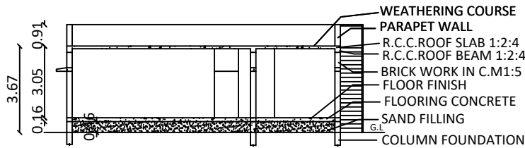
SECTION- SS
