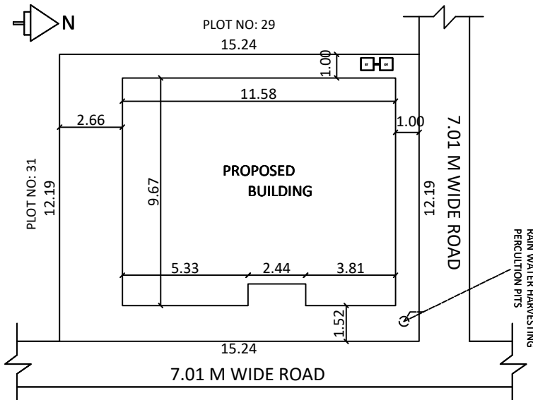
SITE PLAN
