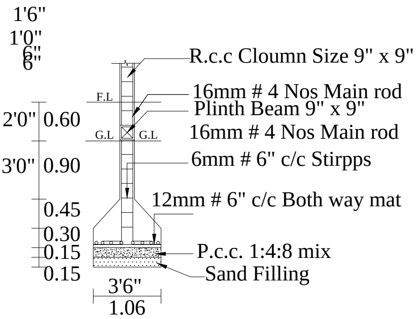
COLUMN DETIAL
