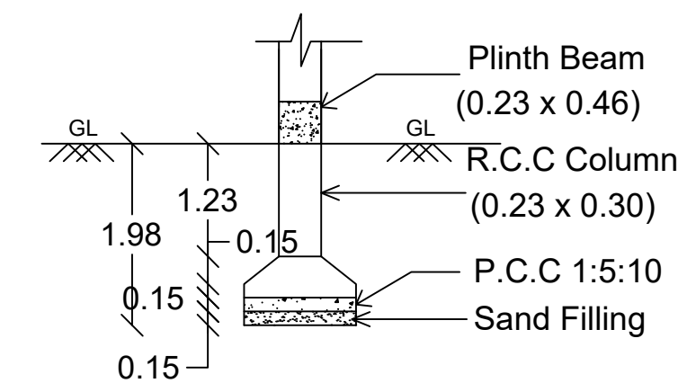
FOUNDATION DETAILS ( Scale 1:100 )
