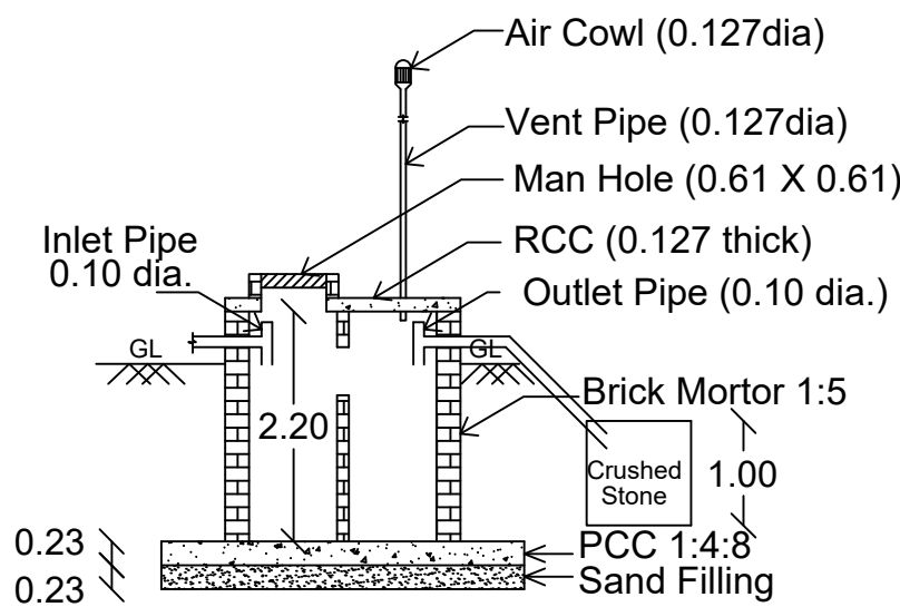
SECTION
