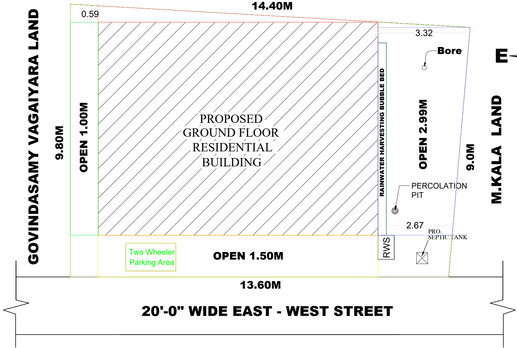
SITE PLAN (SCALE 1:1)
