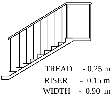
STAIRCASE DETAILS
