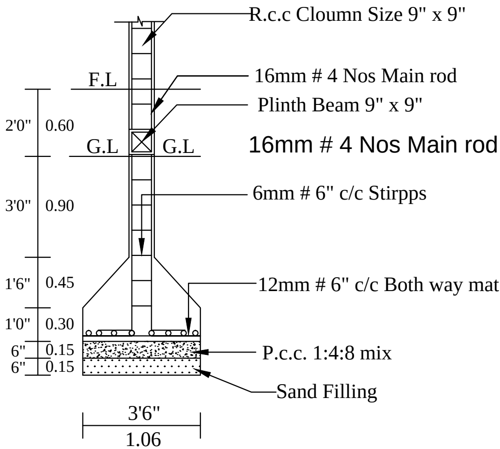
COLUMN DETIAL
