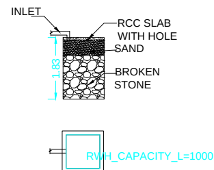
PLAN OF RWH
