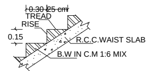
SECTION OF STAIRCASE
