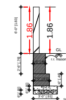
COMPOUND WALL
