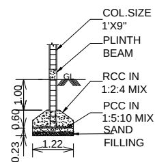
COLUMN DETAILS
