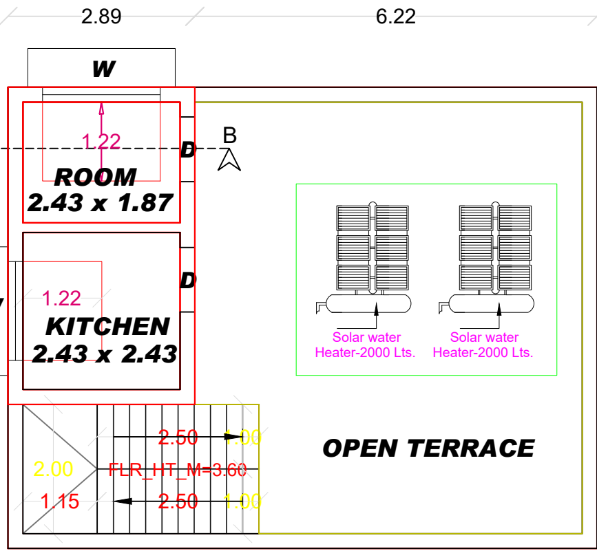
FIRST FLOOR PLAN & OPEN TERRACE PLAN
