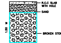
RAIN WATER HARVEST COLLECTION PIT.
