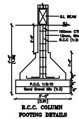
R.C.C. COLUMN FOOTING DETAILS SCALE : 1:20
