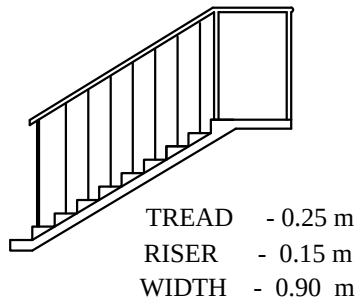
STAIRCASE DETAILS
