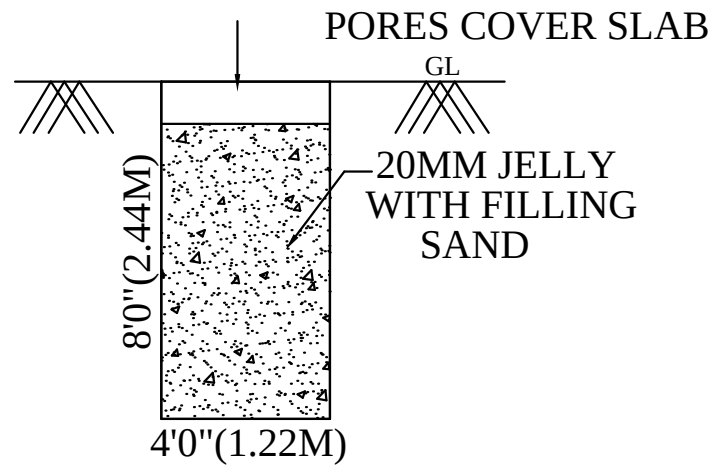
RAINWATER HARVESTING UNIT
