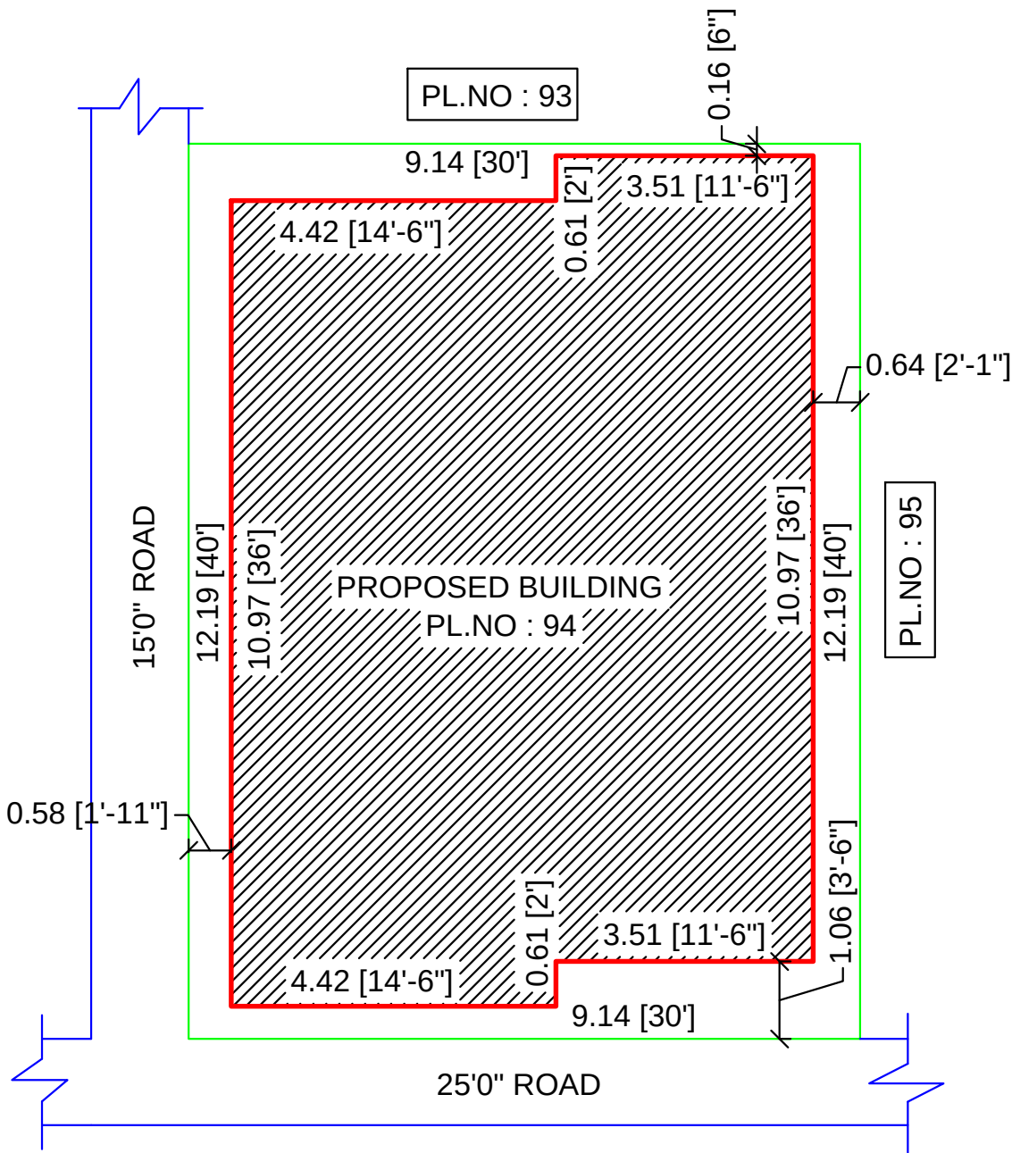
SITE PLAN (1:100)
