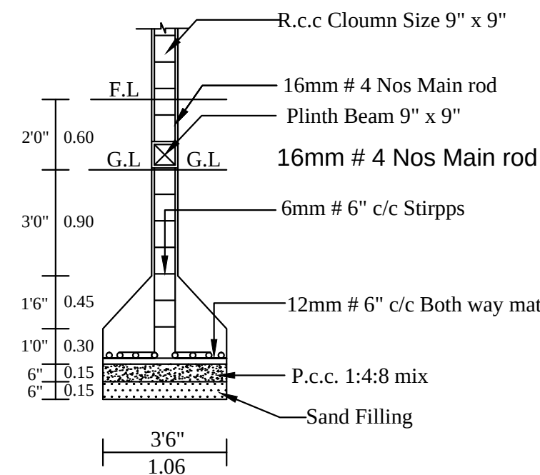
COLUMN DETIAL
