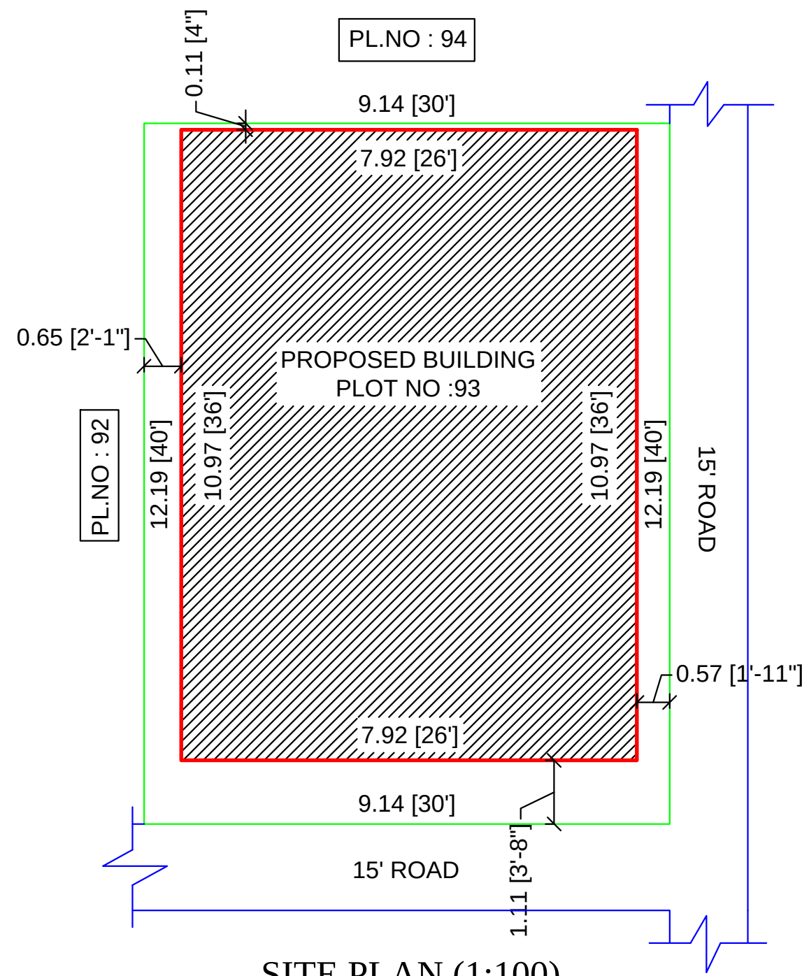
SITE PLAN (1:100)
