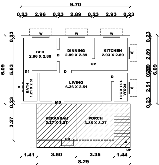
EXISTING GROUND FLOOR PLAN (AS PER MANUAL AUTHORIZED BUILDING PLAN APPROVAL)
