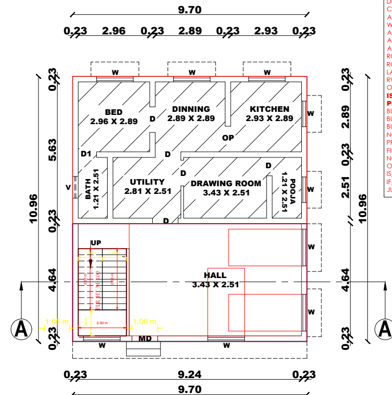
PROPOSED GROUND FLOOR EXTENSION PLAN (AS PER TNCD BR RULES 2019, TAMIL NADU SINGLE WINDOW PORTAL)
