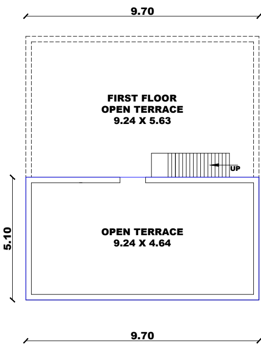
PROPOSED OPEN TERRACE PLAN (AS PER TNCD BR RULES 2019, TAMIL NADU SINGLE WINDOW PORTAL)
