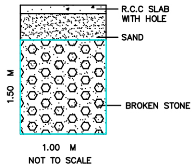
RAIN WATER HARVEST COLLECTION PIT.
