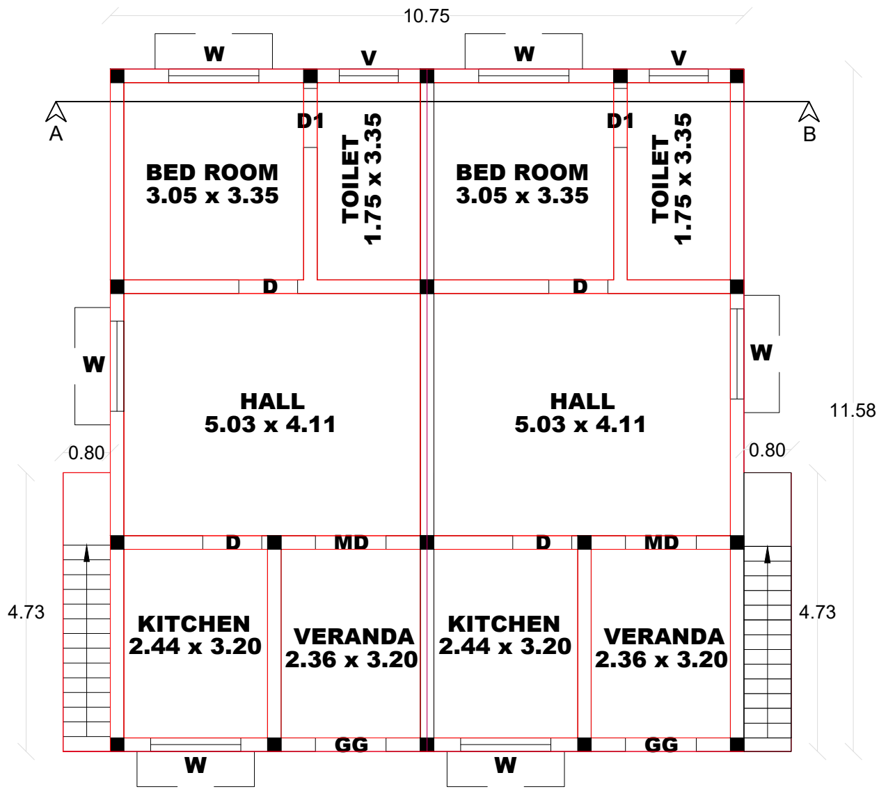
LOOR PLAN
